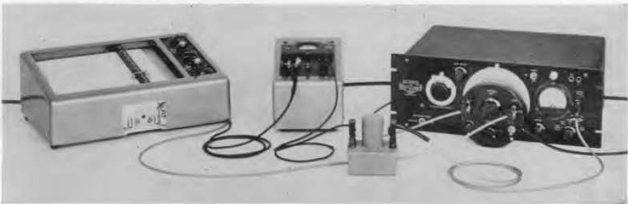
Figure 5. View of the Type 1304-B Best-Frequency Audio Generator and X-Y Dial Drive, with Moseley Model 60 Logarithmic Amplifier and Model 3 Autograph X-Y Recorder, arranged to measure the audio network shown in the foreground. The logarithmic amplifier, whose d-c output is proportional to the logarithm of the a-c input, permits the use of an amplitude scale linear in db.
