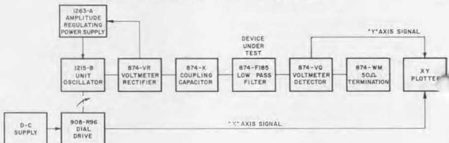
Figure 3. Block diagram for equipment shown in Figure 2.
