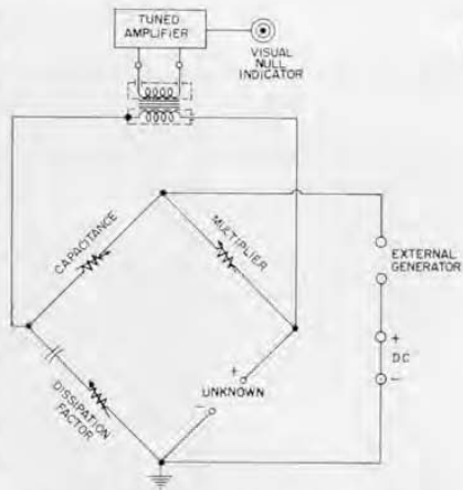
Figure 2. Elementary schematic of the bridge.
