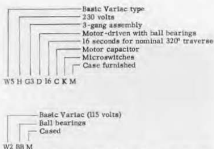
Figure 4. Two examples of how Variac type numbers are formed.
